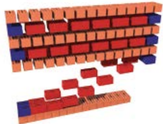
Blockverband
